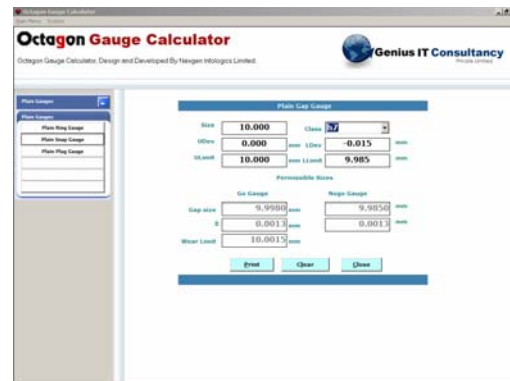
Plain Plug Gauge IS 3455
