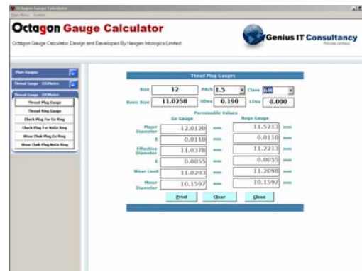
Thread Plug Gauge
