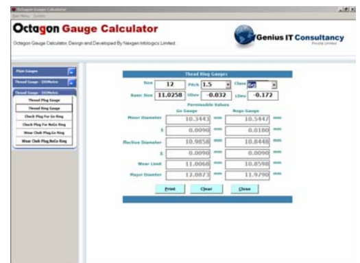
Thread Ring Gauge
