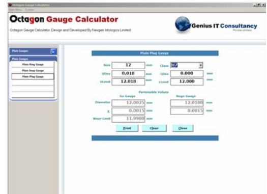
Plain Snap Gauge IS 3455.
